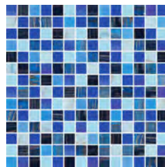
Lamu Dark Blue Size 300 x 300 x 4 mm.
